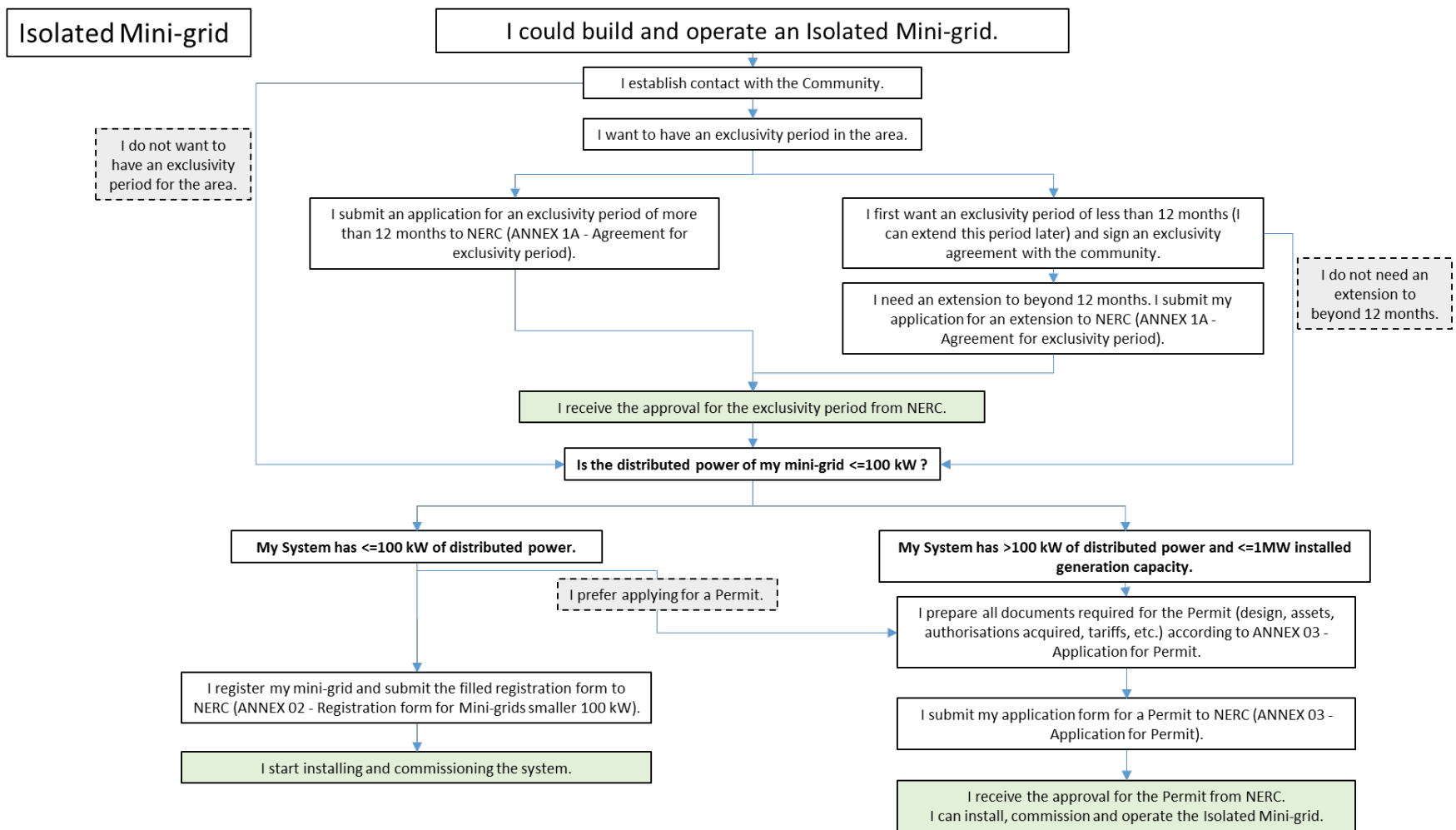
Figure 2: Isolated Mini-Grid
